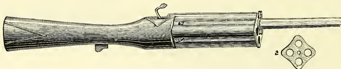
Revolving Arquebus in the Tower of London
